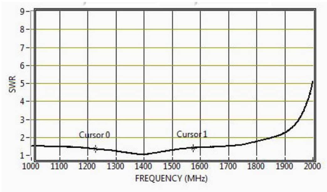
Figure 6. SWR vs. Frequency for Active MS12 Splitter
