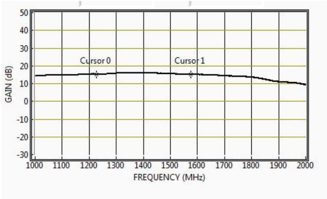
Figure 5. Gain vs. Frequency for Active MS12 Splitter
