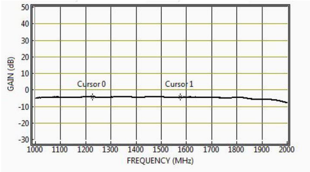
Figure 3. Gain vs. Frequency for Passive MS12 Splitter
