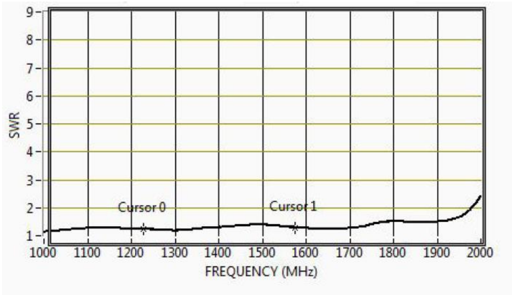
Figure 4. SWR vs. Frequency for Passive MS12 Splitter
