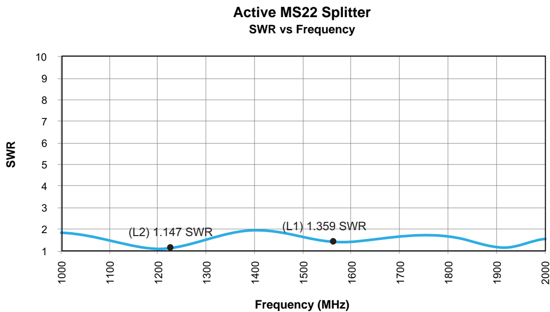
Figure 2-4. Active MS22 Splitter: SWR vs. Frequency
