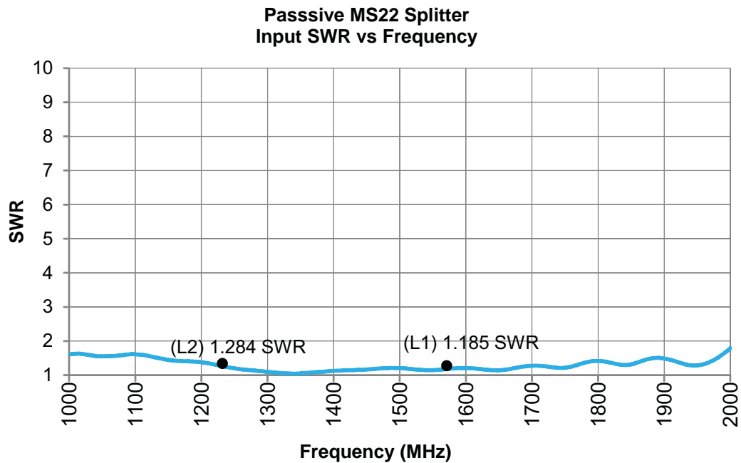
Figure 2-2. Passive MS22 Splitter: Input SWR vs. Frequency
