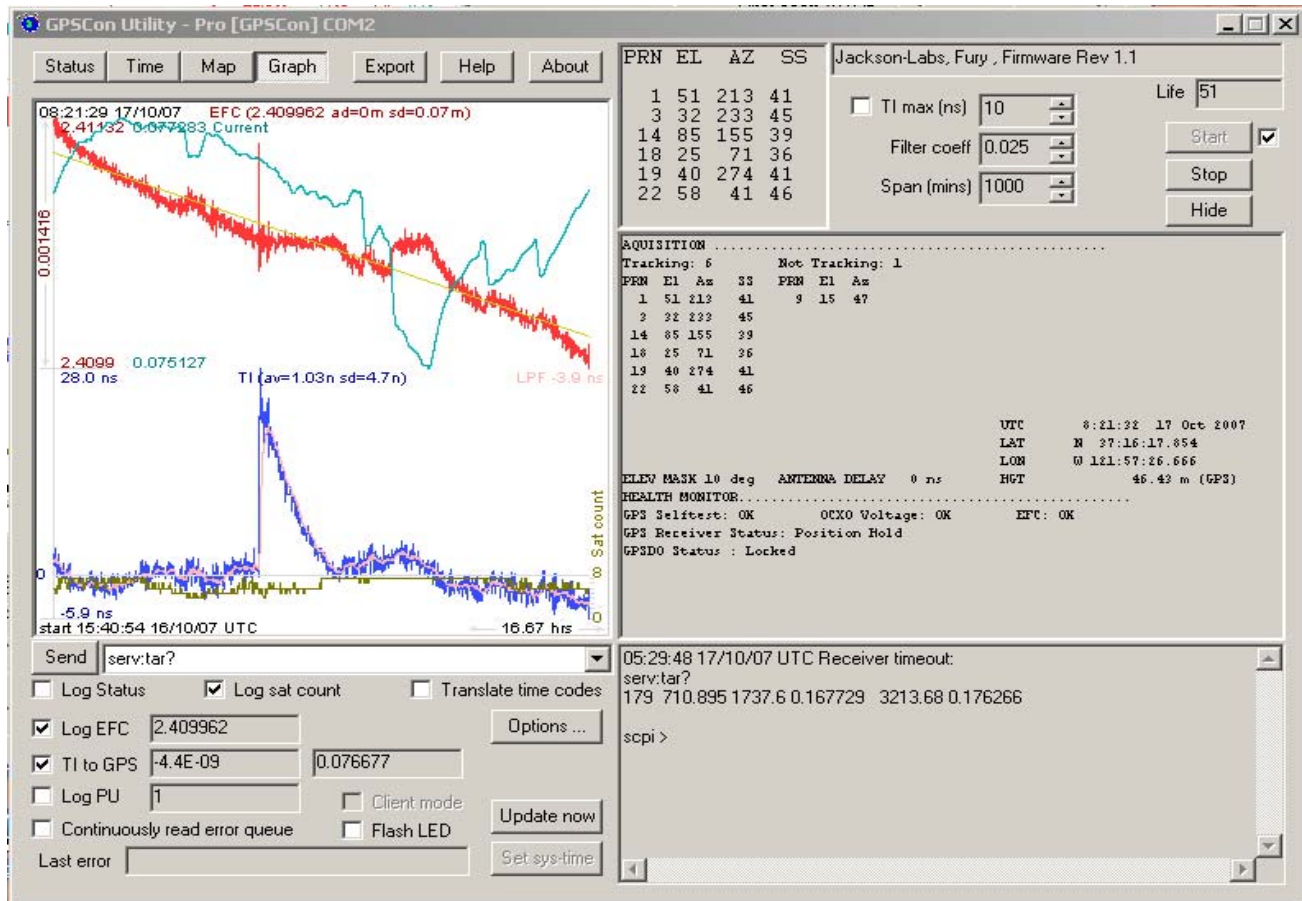
Figure 2.3 HD CSAC Low Power GPSDO phase compensation plot
