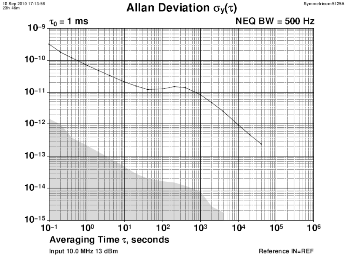
Figure 2.4 Allan Deviation of CSAC when locked to GPS
