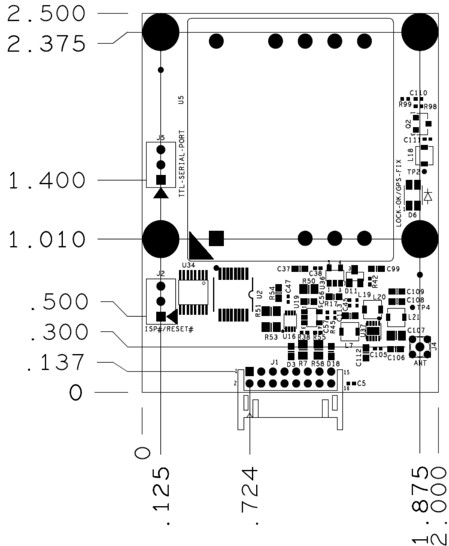
Figure 2.2 HD CSAC Low Power GPSDO Mechanical Drawing
