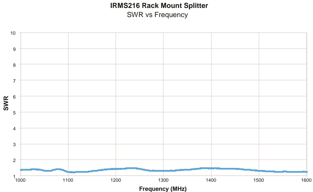
Figure 2-2. IRMS216 Splitter: SWR vs. Frequency
