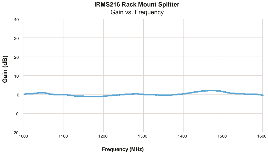
Figure 2-1. IRMS216 Splitter: Gain vs. Frequency
