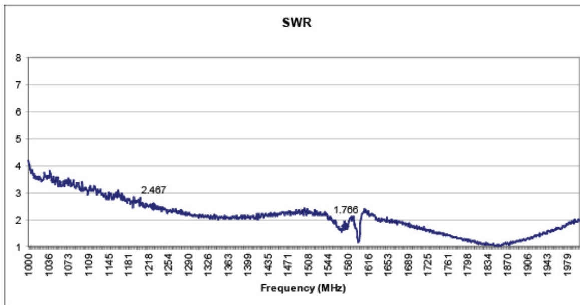
Figure 2-4. Filtered SWR
